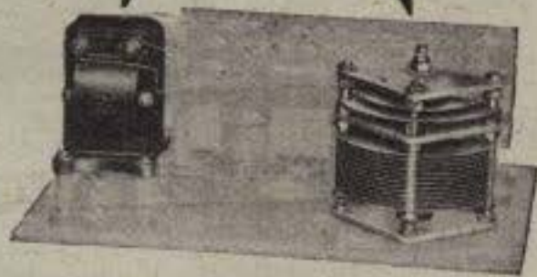
The relative positions of the transformer and condenser are shown in the above photograph. Care in wiring up, disposition of parts, and the use of the two components mentioned are responsible for the perfect functioning of this receiver, especially when used with B.T.H. Valves.
